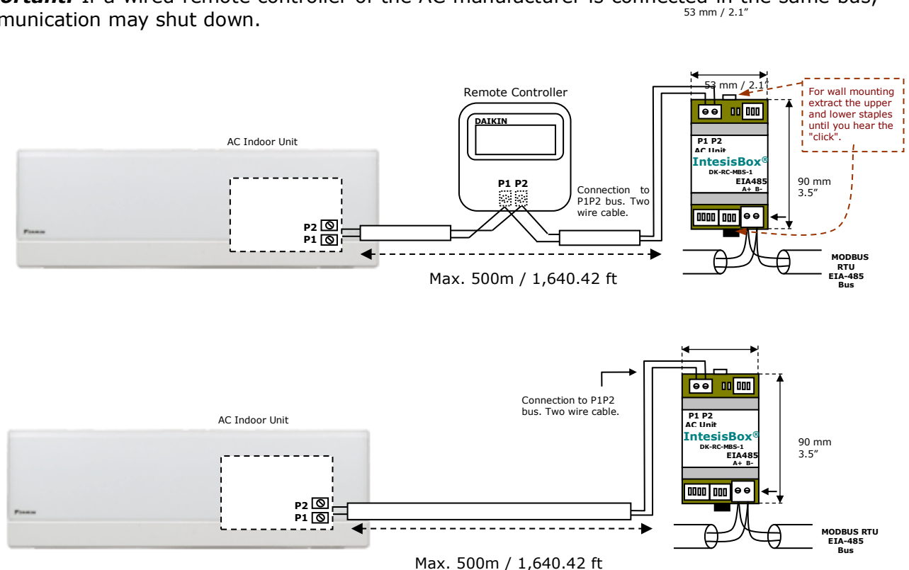
Figure 2. 1 DK-RC-MBS-1 Connection diagrams
