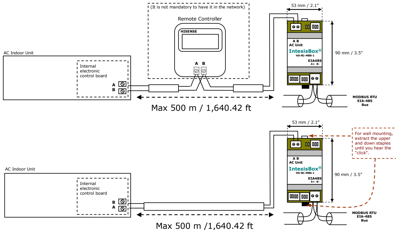
Figure 2. 1 HS-RC-MBS-1 connection diagram
