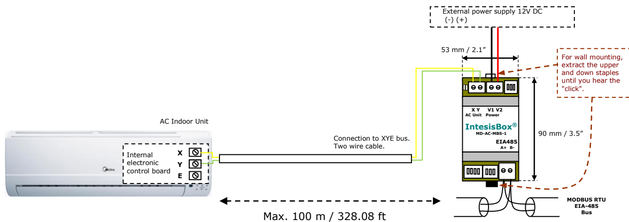
Figure 2.1 MD-AC-MBS-1 connection diagram
