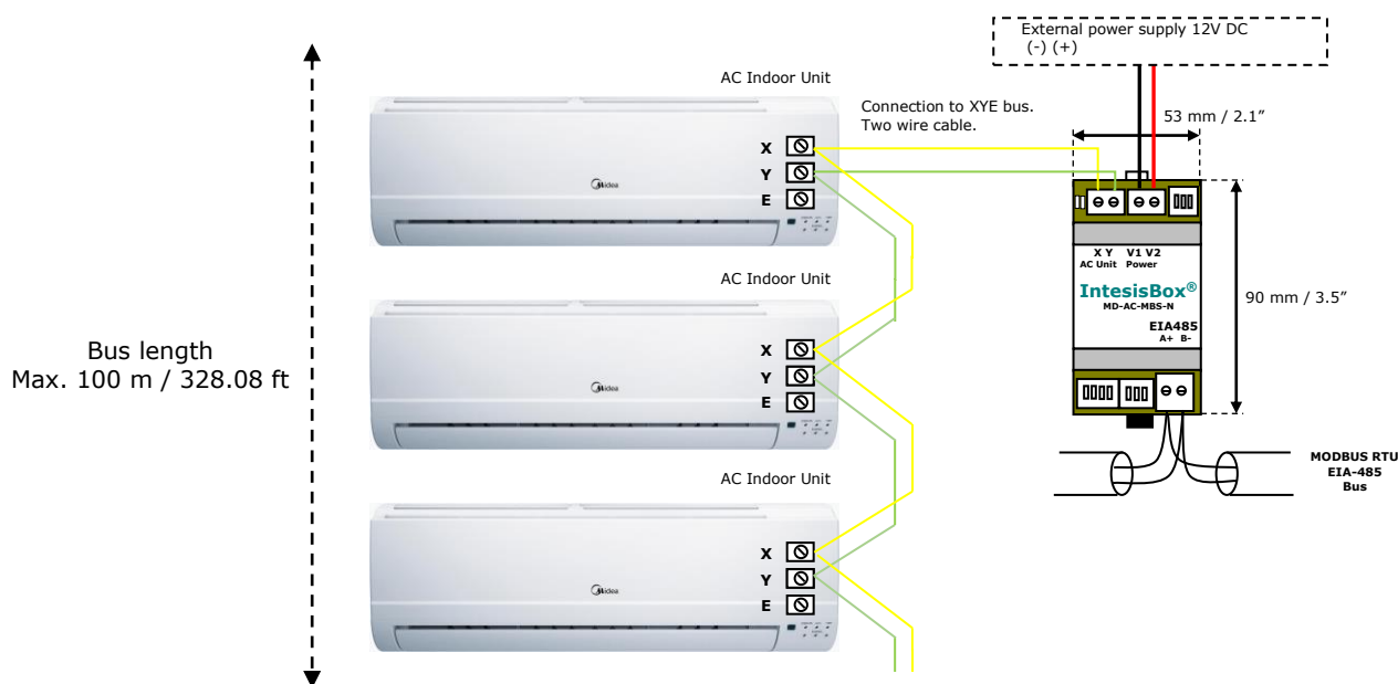
Figure 2.2 MD-AC-MBS-4/8/32 connection diagram
